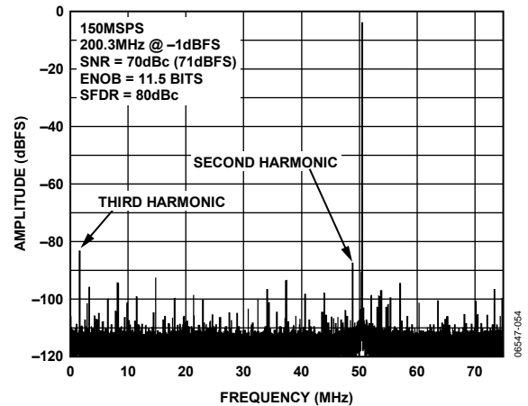
Figure 20. AD9640-150 Single Tone FFT with f_{IN} = 200.3 MHz
